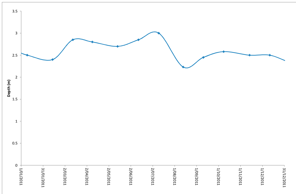
Figure 47. Water depth at site P2 during 2011.
