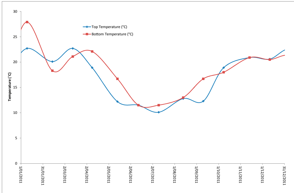
Figure 48. Temperature (top and bottom) at site P2 during 2011.
